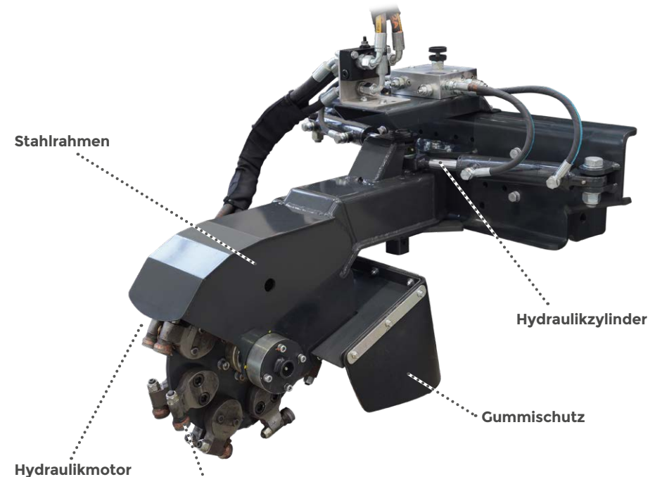
Hydraulikmotor
